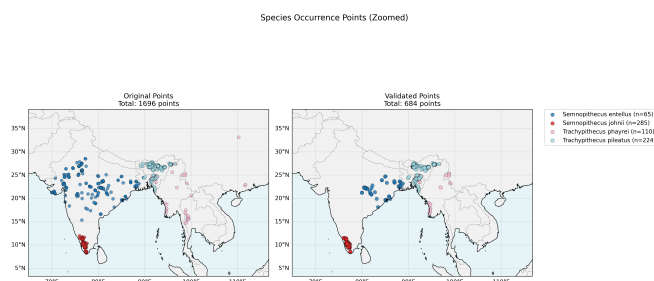
Fig. 5. Detailed view of occurrence point clustering highlighting regions where multiple langur species co-occur, supporting observed introgression patterns.
