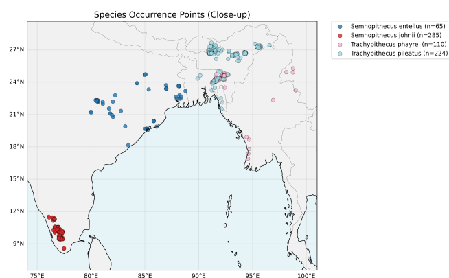
Fig. 4. Geographic distribution of occurrence points showing species range overlaps and potential contact zones that enable hybridization.
